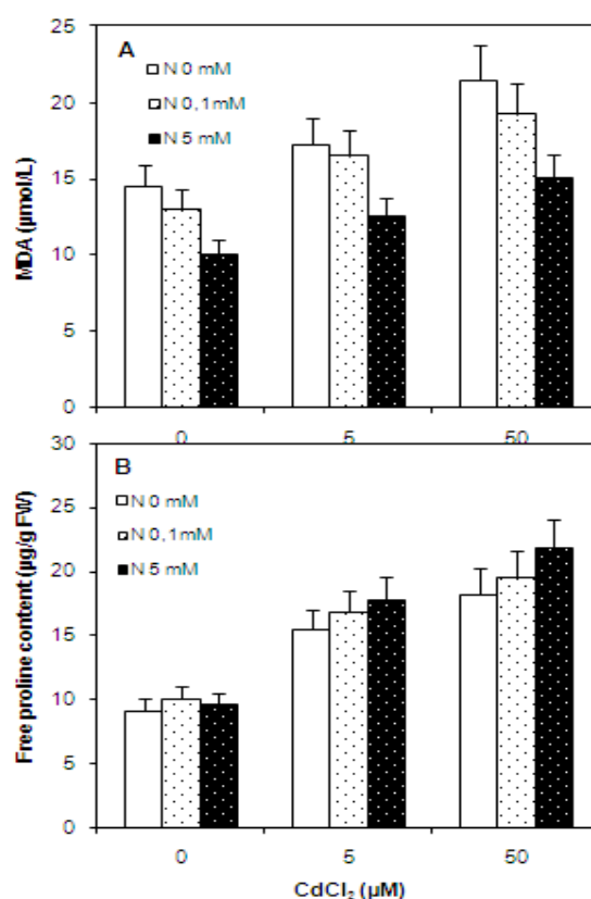
Fig. 4. Interactive effect of Cd and N treatment on MDA and free proline content in N. tabaccum , (A) MDA content, (B) Free proline content.
