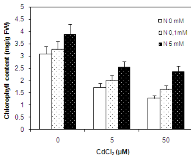
Fig. 2. Interactive effects of Cd and N treatment on chlorophyll contents in N. Tabaccum .
