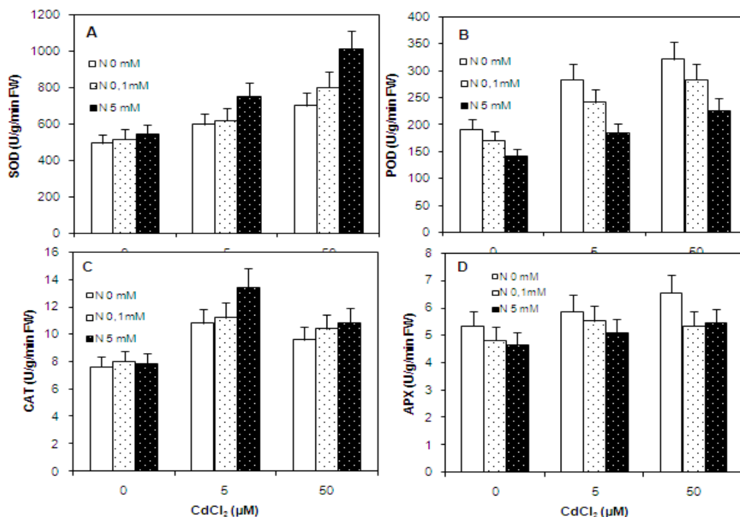
Fig. 3. Interactive effects of Cd and N treatment on antioxidant enzymes activities of N. tabaccum , (A) SOD activities, (B) POD activities, (C) CAT activities, (D) APX activities.
